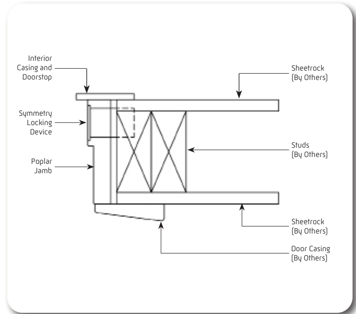
Flush door frame for SLD detail
