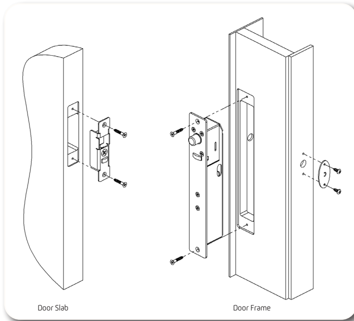
Symmetry Locking Device detail
